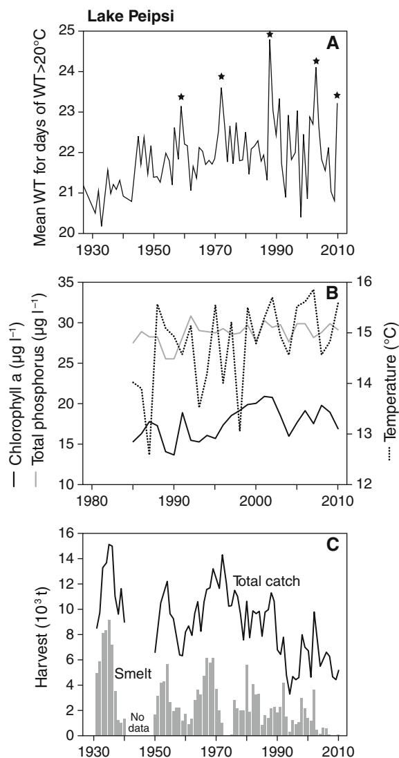
Fig. 5 Lake Peipsi. A Mean water temperature (WT) for days with temperature >20^{\circ}\text{C} from 1925 to 2010. The occurrences of fish kills during the hottest summers are marked with asterisks . B Mean water temperature, total phosphorus and chlorophyll a for the ice-off period. C Annual catches of smelt and total fish
