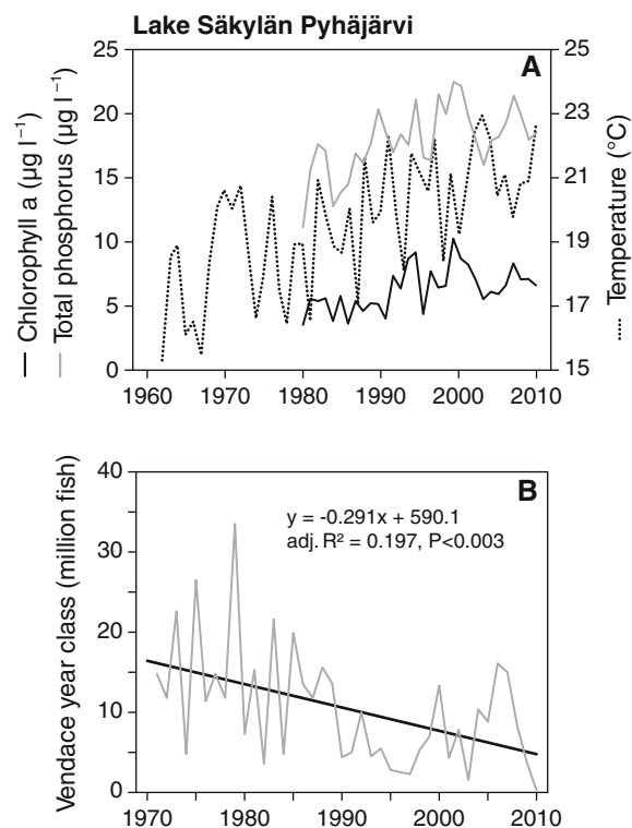
Fig. 4 Lake Säkylän Pyhäjärvi. A Mean total phosphorus, chlorophyll a (0–5 m; May–September) and annual maximum water temperature. B Year class size of vendace (in millions)
