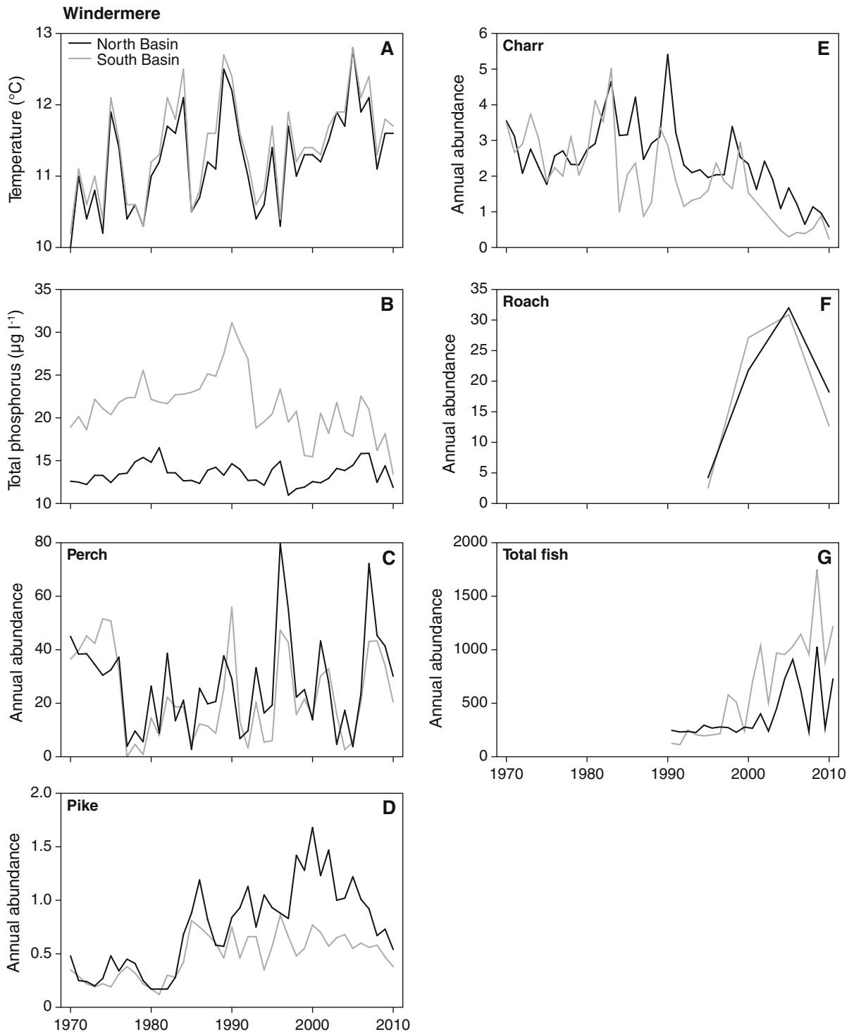
Fig. 8 Windermere. A Annual mean surface water temperature in the north and south basins. B Annual mean total phosphorus in the north and south basins. C–F Annual abundance of perch (fish trap ^{-1} week ^{-1} ), pike (fish net ^{-1} day ^{-1} ), Arctic charr (fish
